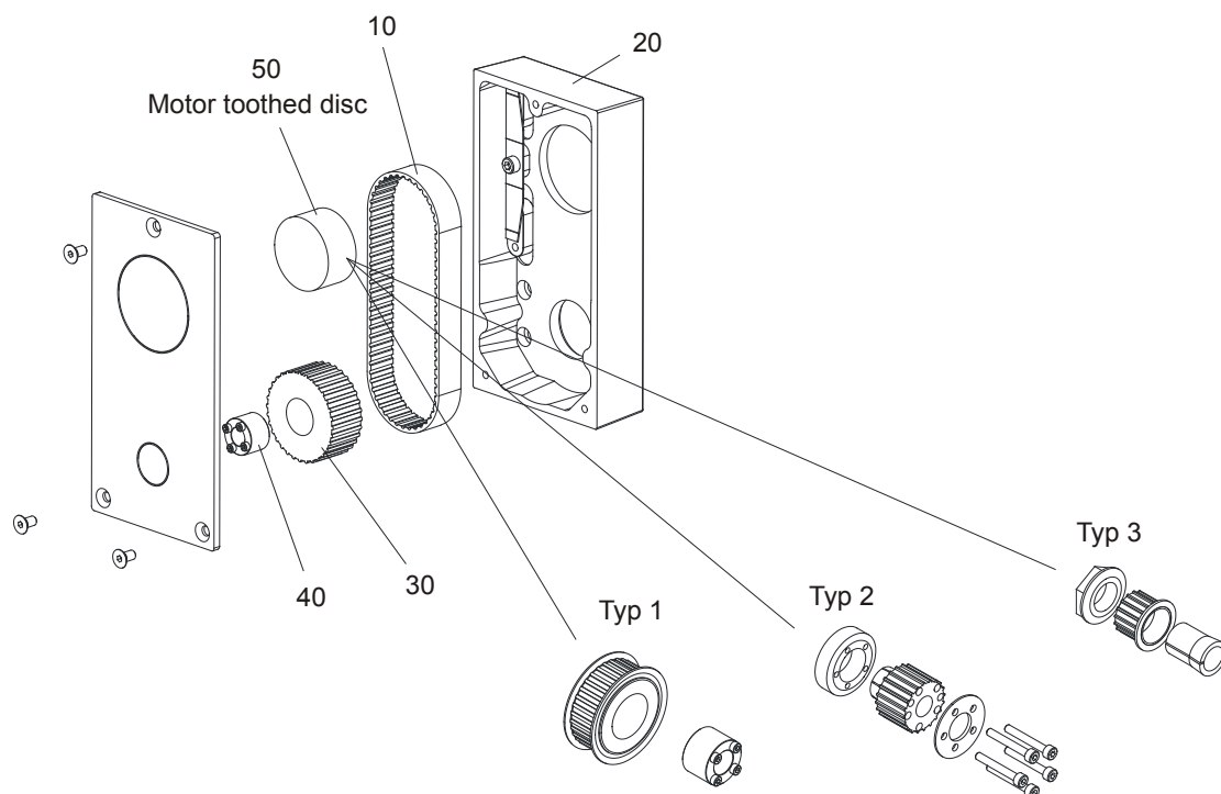
Figure 24: easyLINE, gearbox exploded view
