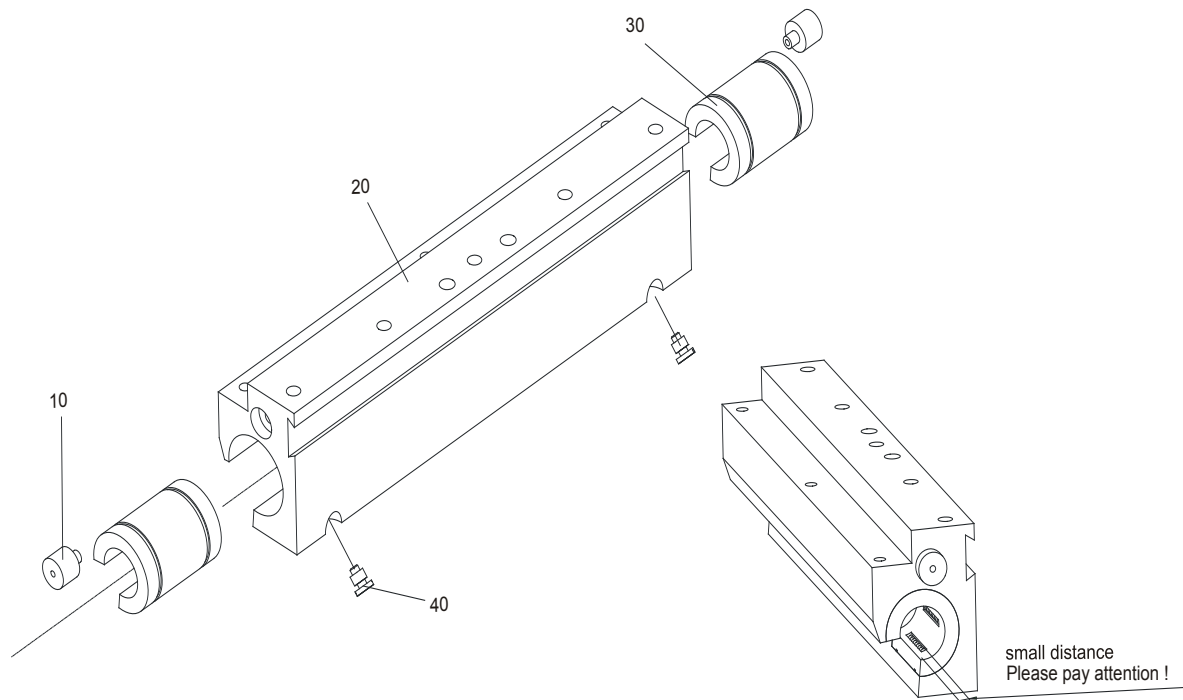
Figure 27: easyLINE long slide clamping block complete
