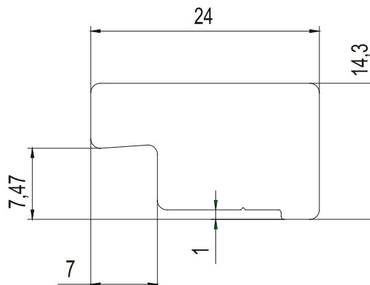
Figure 6: Dimensions clamping element
